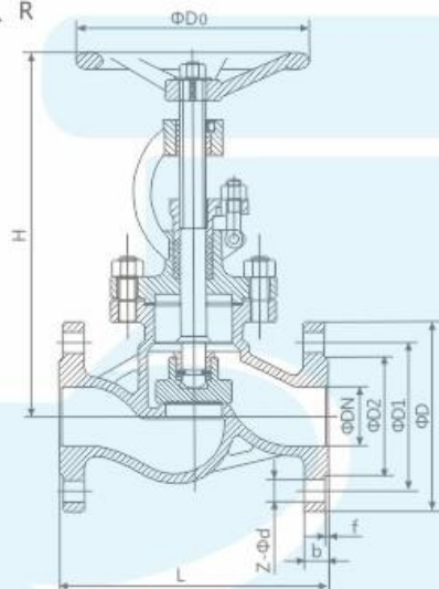
PN16 Main external and connection dimension
