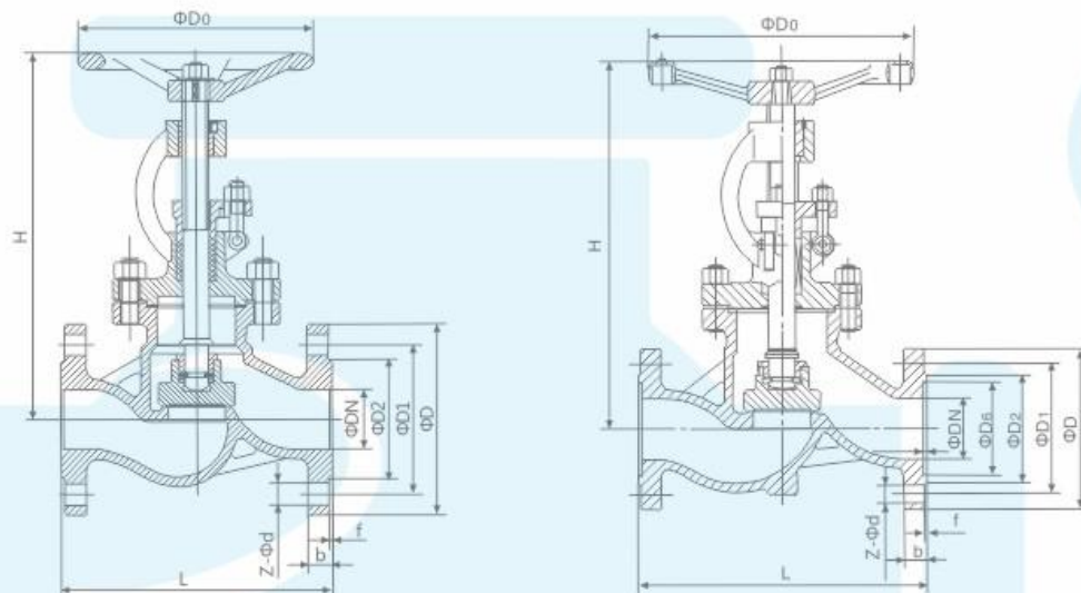
PN16 Main external and connection dimension
